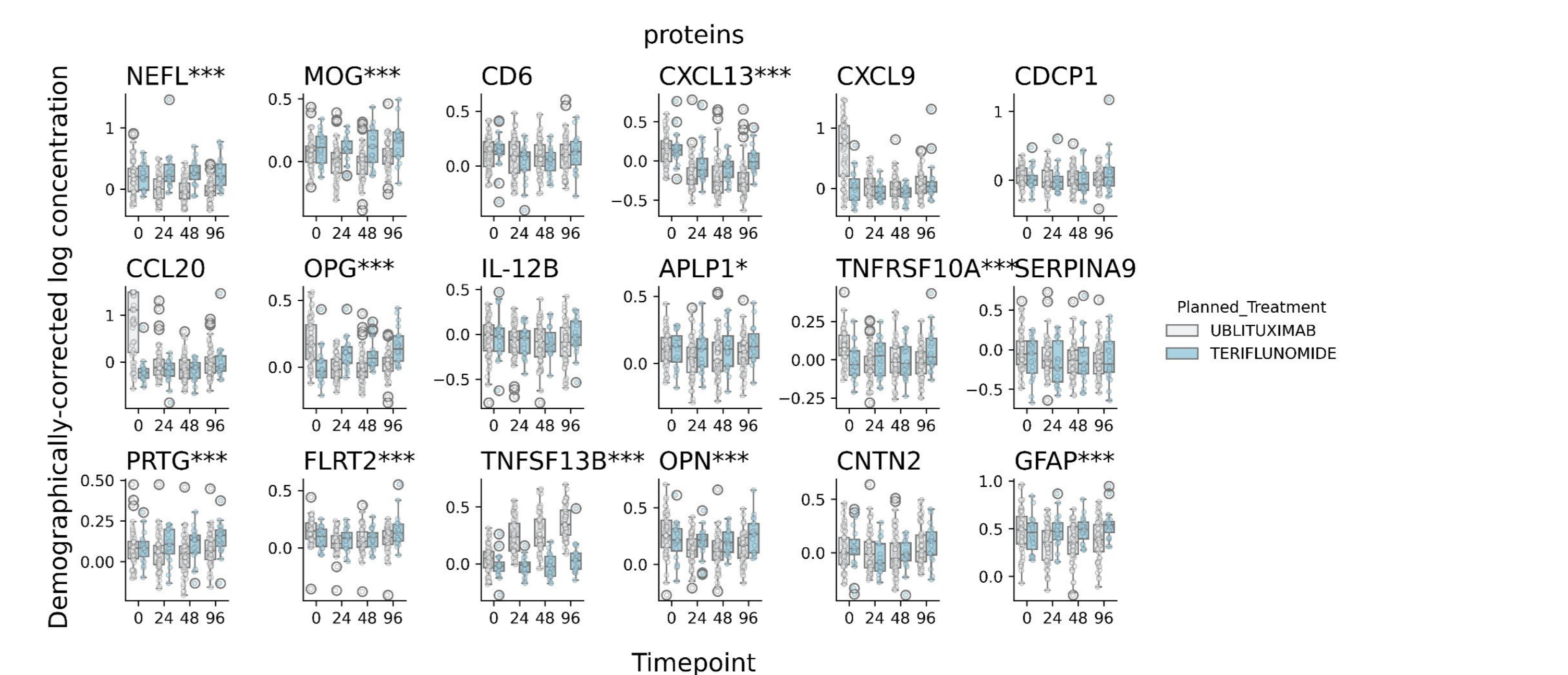
Figure 2: Boxplots of the 18 protein log concentrations (after demographic correction) over the 4 different timepoints (0, 24, 48, 96 months) by treatment arm. * = nominally significant, *** = significant after Bonferroni correction
